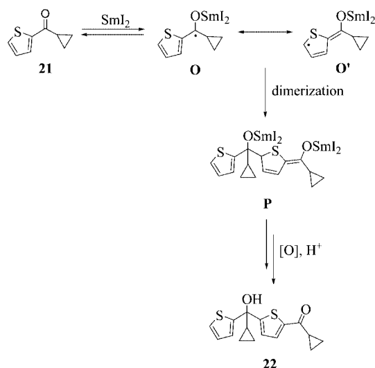
Scheme 9.
